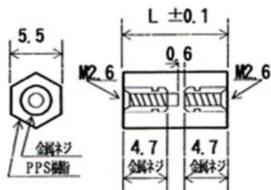
PS2.6 A (M2.6 P-0.45)
