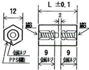
PS8A (M8 P=1.25)
