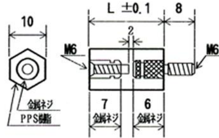
PS6B (M6 P=1)
