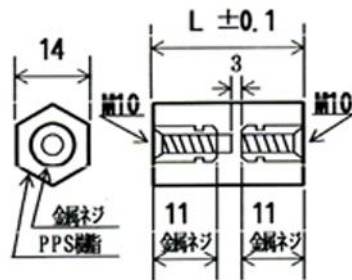
PS10A (M10 P=1.5)
