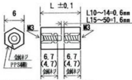
PS3A (M3 P-0.5)
