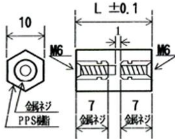
PS6A (M6 P=1)
