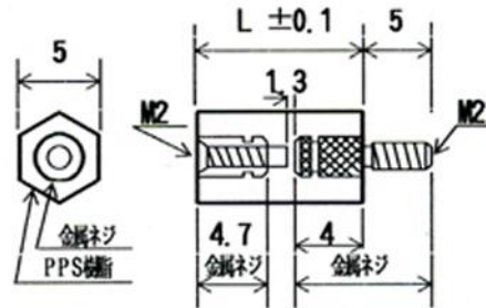
PS2B (M2 P=0.4)
