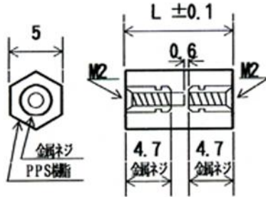
PS2A (M2 P=0.4)
