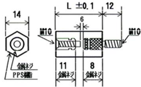
PS10B (M10 P=1.5)
